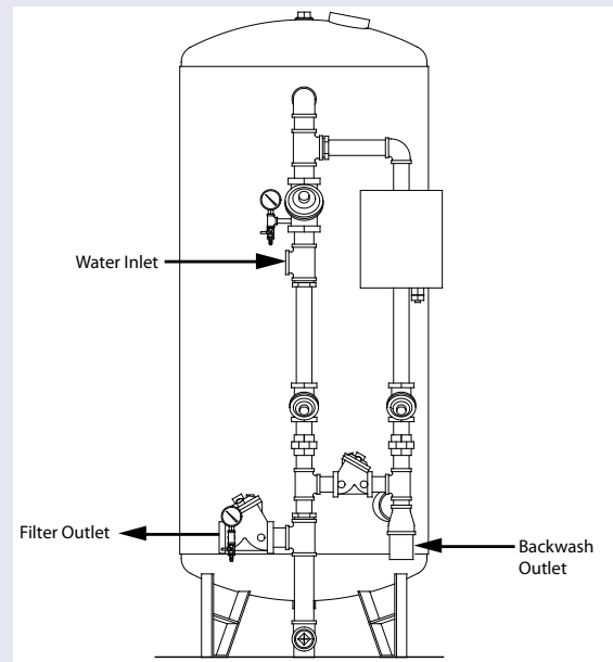
BWS54 Series filtering system.
